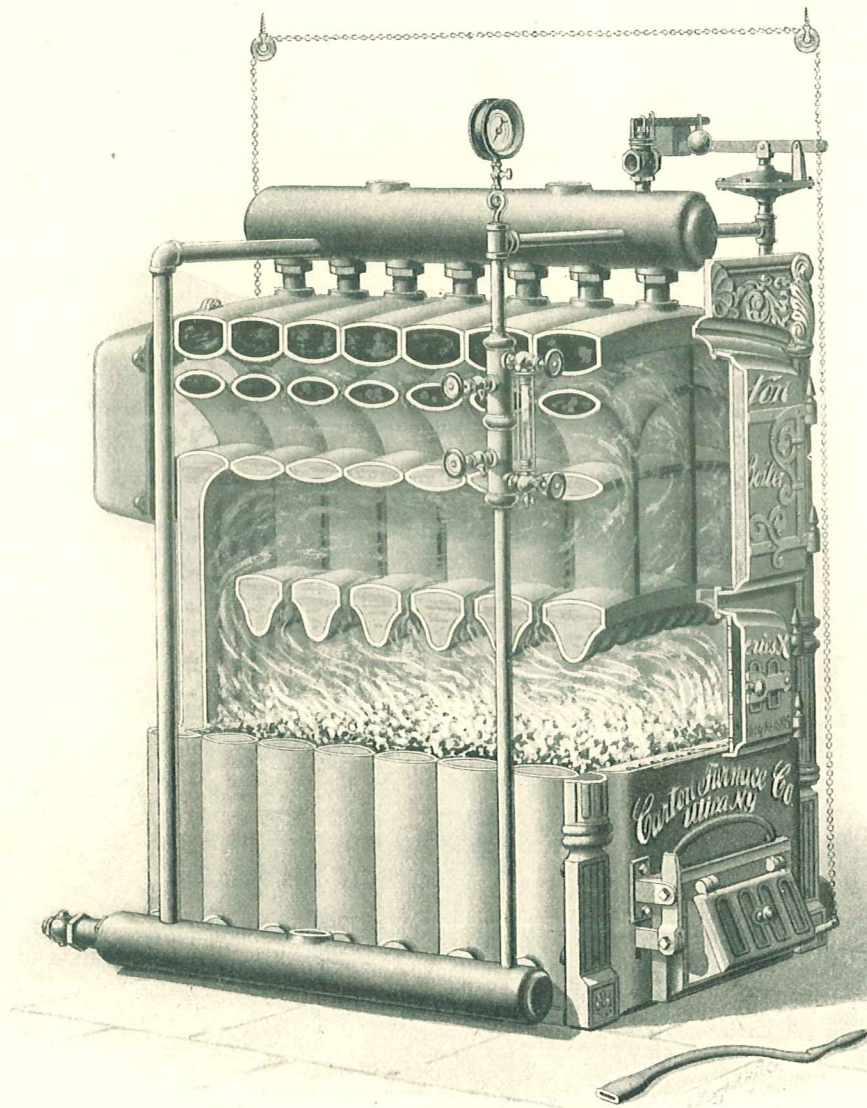
"A" Series Carton Steam Boiler. Cut Away View.
