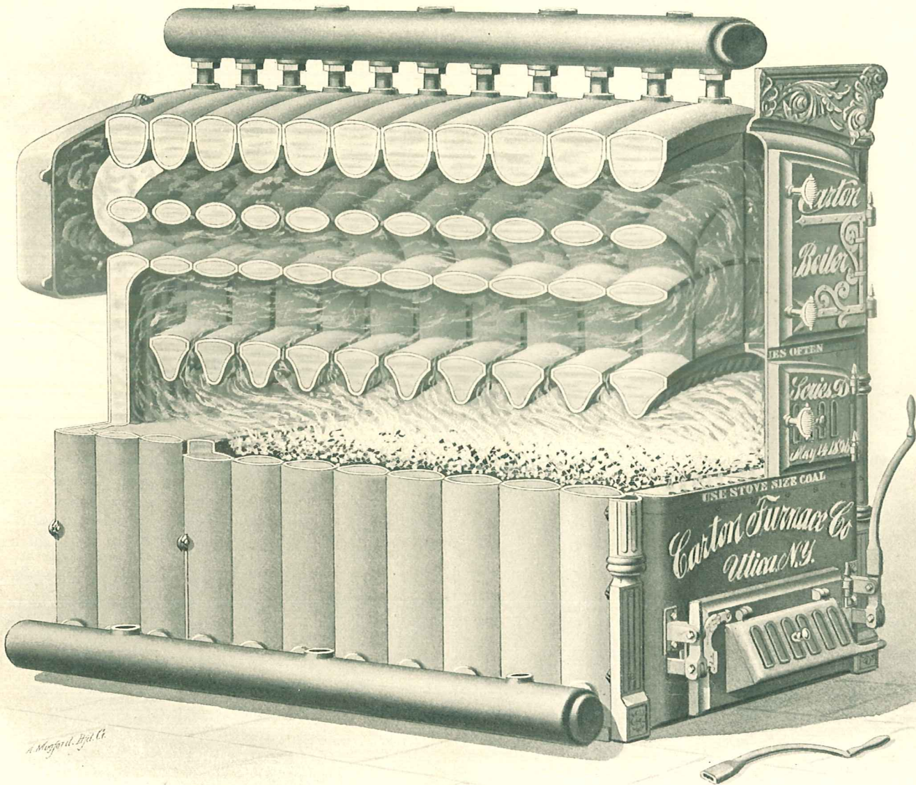
"D" Series Carton Hot Water Boiler. Cut Away View.
